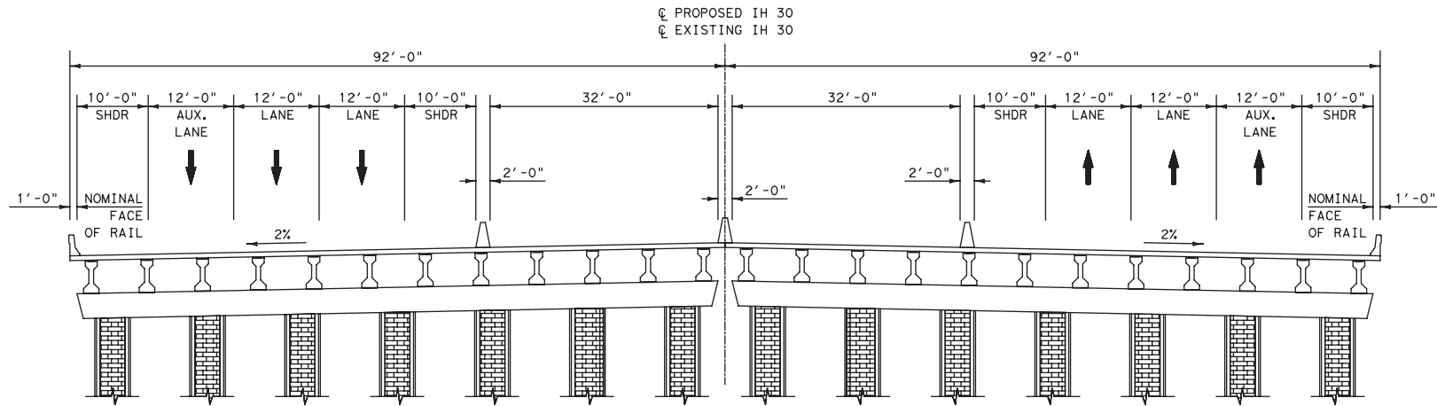
PROPOSED IH 30 BRIDGE SECTION
