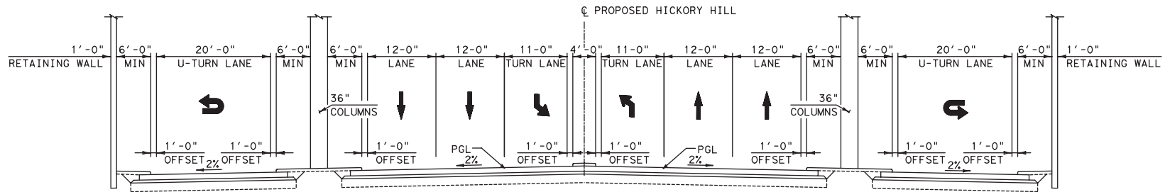
PROPOSED HICKORY HILL ROADWAY SECTION
